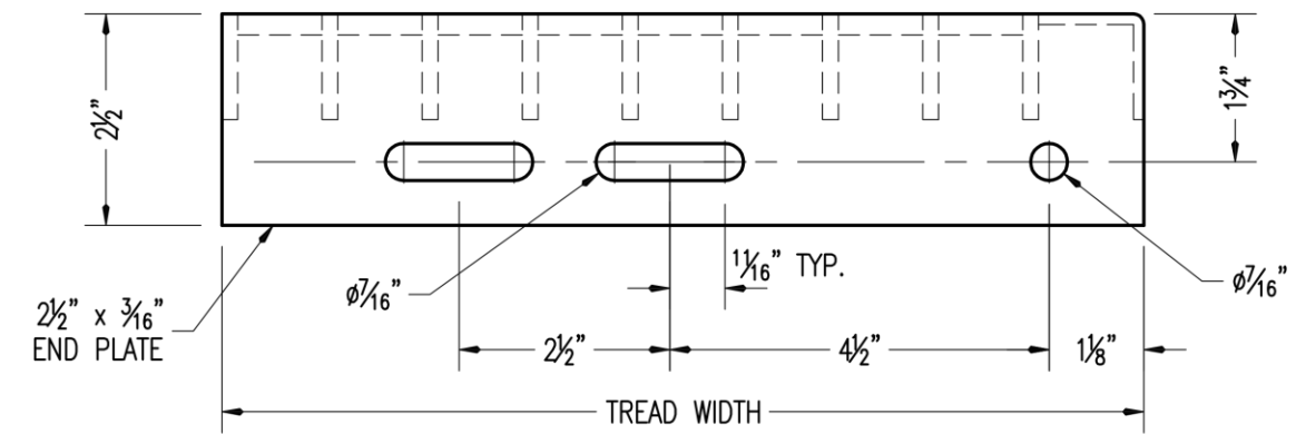
2 1/2" STANDARD END PLATE STEEL OR ALUMINUM
