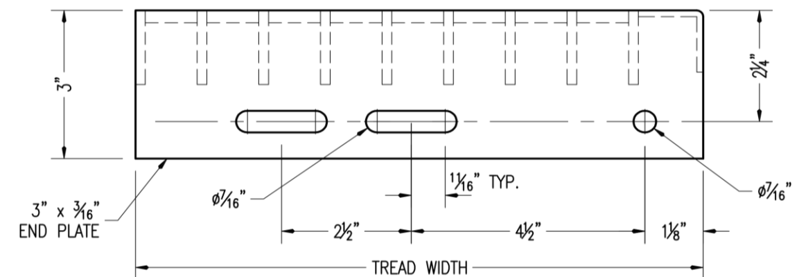
3" STANDARD END PLATE STEEL OR ALUMINUM
