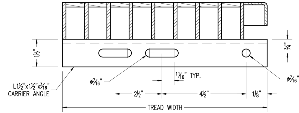
CARRIER ANGLE STEEL OR ALUMINUM
