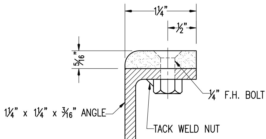
CAST ABRASIVE NOSING (ALUMINUM) FOR STEEL OR ALUMINUM TREADS
