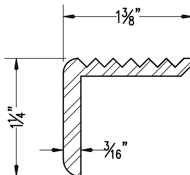
CORRA-TRED NOSING (ALUMINUM) FOR ALUMINUM TREADS ONLY
