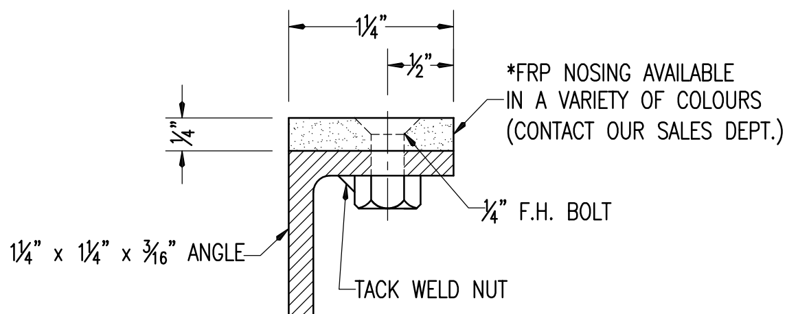
FRP ABRASIVE NOSING (FRP) FOR STEEL OR ALUMINUM TREADS
