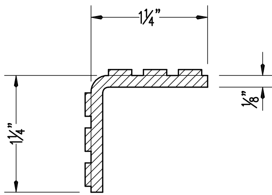
CHECKERED PLATE NOSING (STEEL) FOR STEEL TREADS ONLY
